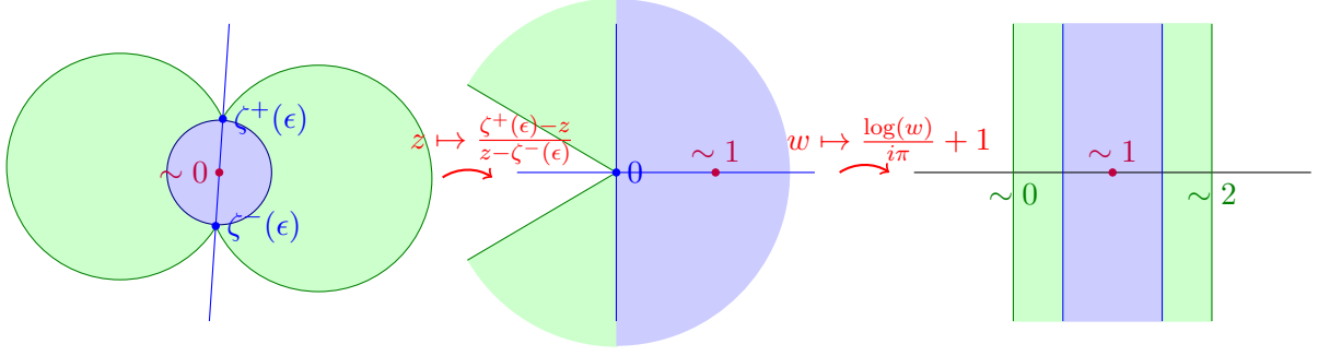
FIGURE 1. The sets D_\epsilon \subset \mathcal{S}(\epsilon, r) and their images under \psi_\epsilon^t .
