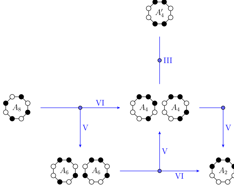
FIGURE 8. Minimal transitions between particle/hole configurations in B_0 for N=8 . Arrows indicate transitions that decrease the energy, and are labelled according to Table 1. Each node displays only one representative of an orbit for the group action of \mathfrak{D}_N \times \mathbb{Z}_2 . The other elements of an orbit are obtained by applying rotations, reflections and interchanging particles and holes. Blue nodes represent stationary points in B_1 . Not shown are transitions within the families A_p and A'_p , which are of type III or IV.
