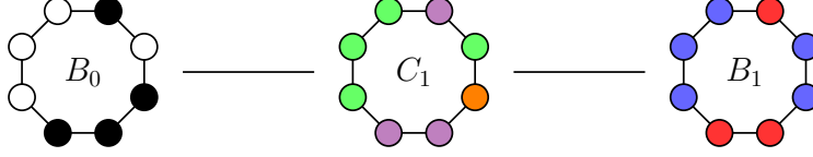
FIGURE 4. Example of transition rules for N = 8 . The coordinates for family B_0 are \bullet = 1 and \circ = -1 . Those for C_1 are \text{orange} = -1/\sqrt{7} , \text{purple} = 3/\sqrt{7} and \text{green} = -2/\sqrt{7} . Those for B_1 are \text{red} = 5/\sqrt{19} and \text{blue} = -3/\sqrt{19} .
