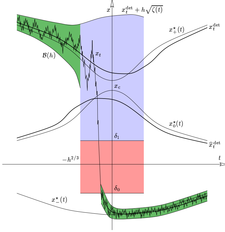
FIGURE 5. A typical path x_t of the SDE (2.1) in the asymmetric case, shown near t = 0 , where the right-hand well at x_+^*(t) approaches the saddle at x_0^*(t) . We show again a situation where the noise intensity is large enough to allow a transition. The deterministic solution x_t^{\text{det}} starting near the right-hand potential well tracks x_+^*(t) at a distance at most of order (\varepsilon/\sqrt{a_0}) \wedge \sqrt{\varepsilon} , and never approaches the saddle at x_0^*(t) closer than \sqrt{a_0} \vee \sqrt{\varepsilon} . The path x_t is likely to stay in the set \mathcal{B}(h) up to time -h^{2/3} when h \gg \sigma . Between times -h^{2/3} and h^{2/3} , the path is likely to reach the saddle. Although it may fall back into the right-hand potential well, it is likely to finally overcome the potential barrier and reach a level \delta_1 of order 1 below the saddle, after which it quickly reaches a lower level \delta_0 . The distance between \delta_1 and \delta_0 can be much larger than in this picture. Finally, the path will track the deterministic solution starting in x = \delta_0 , which approaches a neighbourhood of order \varepsilon of the left-hand potential well at x_-^*(t) .
