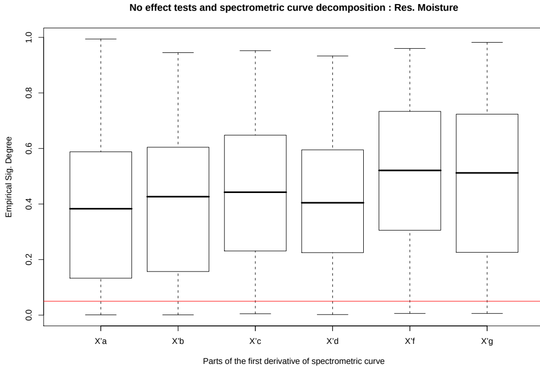
FIGURE 11.13. No effect tests and Spectrometric curves decomposition
