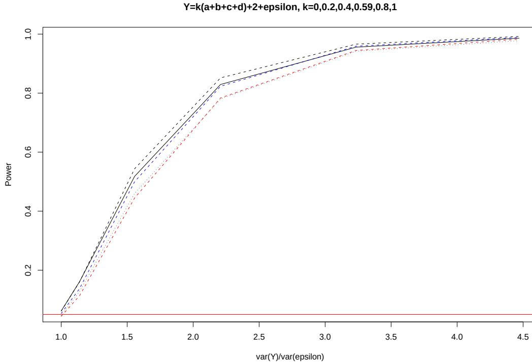
FIGURE 11.2. Power of bootstrap procedures relatively to the value of the signal-to-noise ration R
